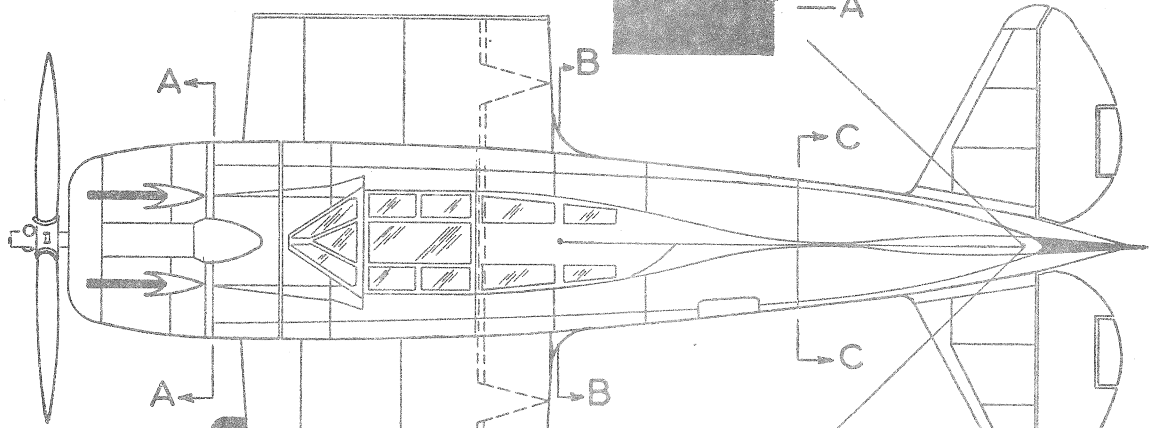
REPUBLIC P-41A A.P. 9 U.S. ARMY PURSUIT PLANE
