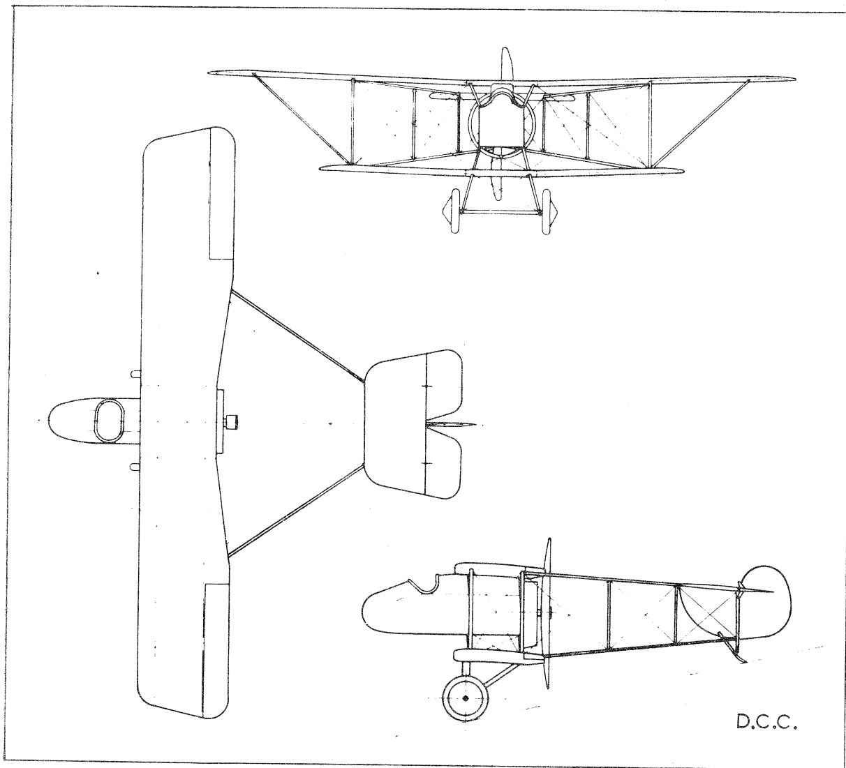
General arrangement drawing of Robey pusher scout.
