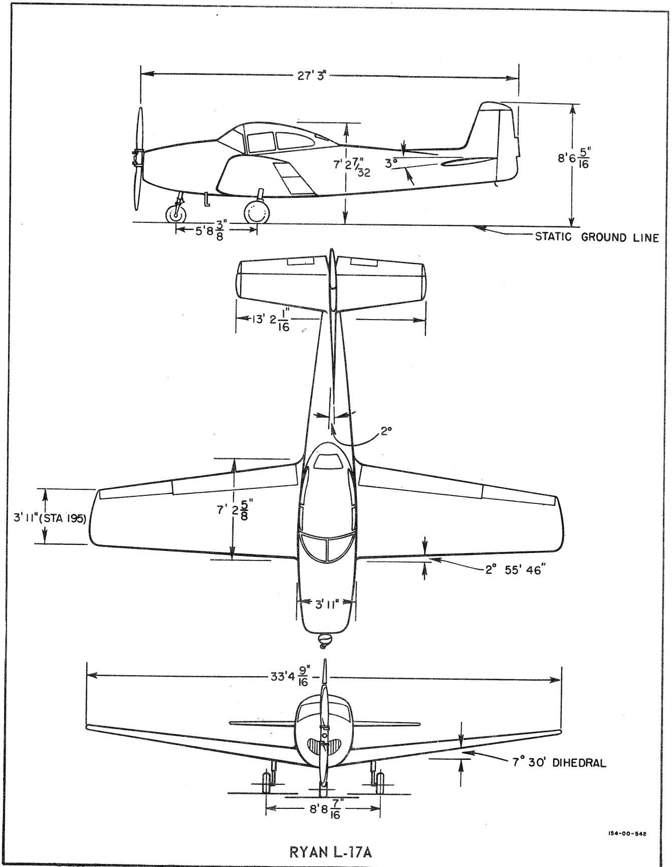
Figure 1-1. Airplane Dimensions
