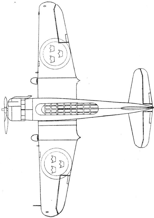
ABOVE, LEFT: The first SAAB-17 prototype (FV serial 17001) was powered by a Mercury XXIV. SAAB-17 variants are shown in the drawing. ABOVE, RIGHT: An earlier dive-bomber was the Northrop 8A-1, built in Sweden as the B 5
