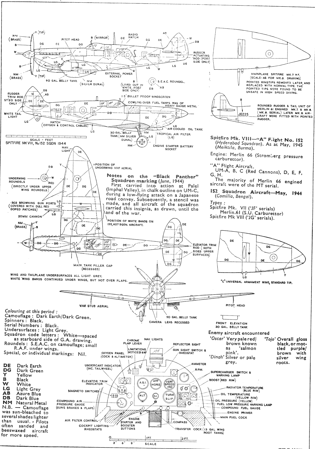
Above drawing by G. R. Duval is of his aircraft as flown in Burma 1944/5 and will be specially helpful to Spitfire modellers.
