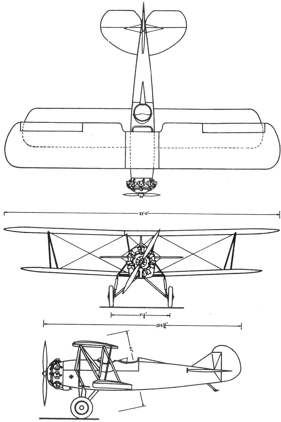
TRAVEL AIR COMPANY Wichita, Kan. MODEL 4 D 3 PLACE ENGINE: WRIGHT WHIRLWIND 220 WRIGHT WHIRLWIND 165
