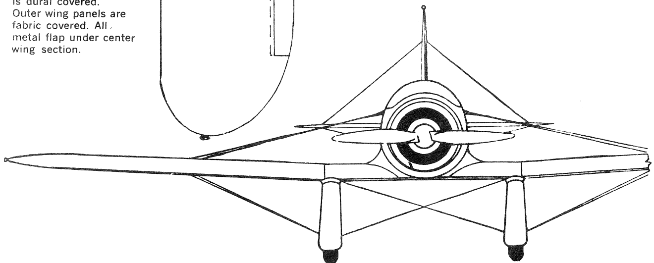
Two place wire braced monoplane
